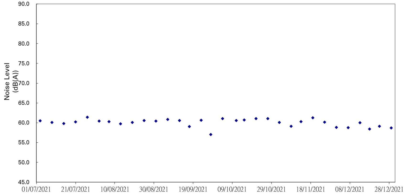
Noise Level (Leq 30 mins) dB(A) Vs Date for Location W-N1A
